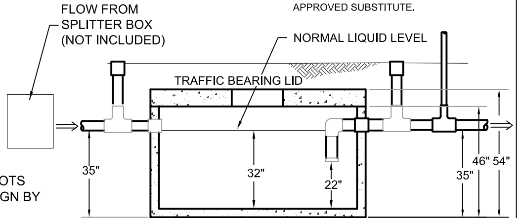
SECTION C-C
